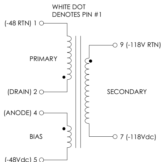
FIGURE 1: SCHEMATIC DIAGRAM
